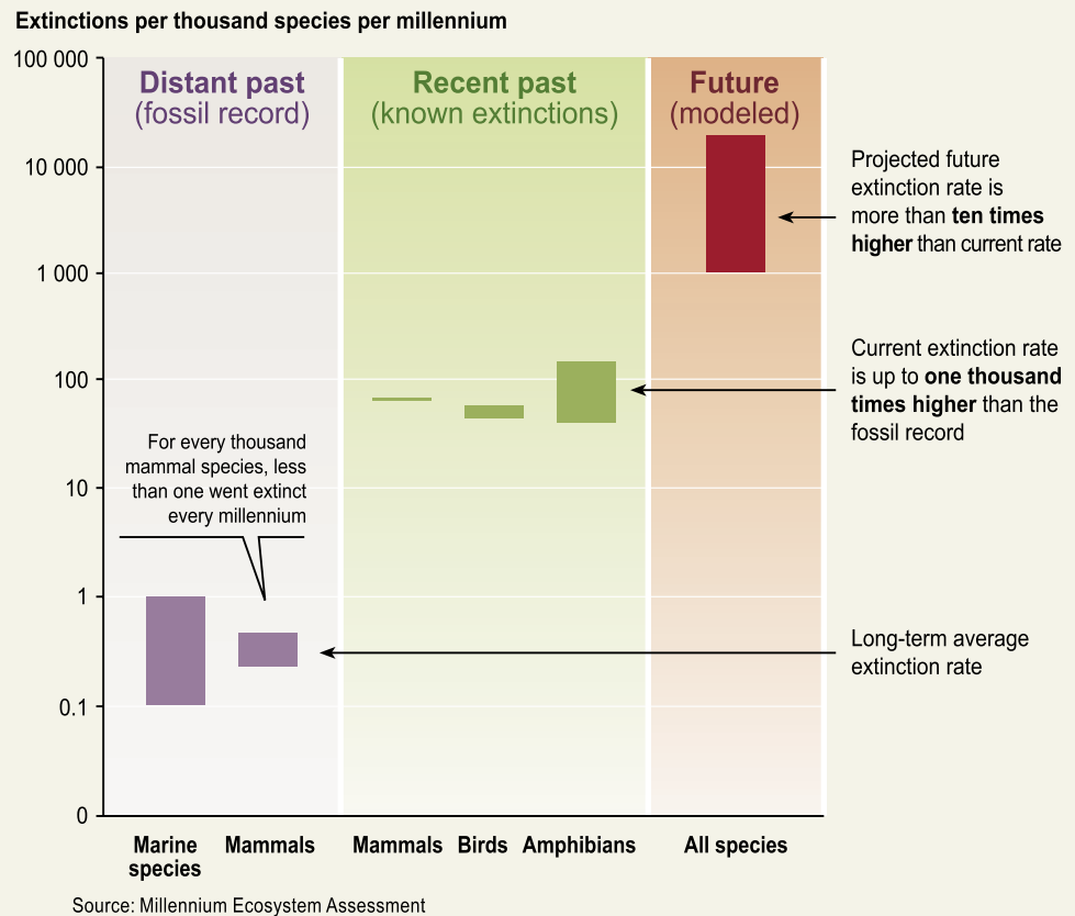
Figure 1.8. SPECIES EXTINCTION RATES (Adapted from C4 Fig 4.22)
