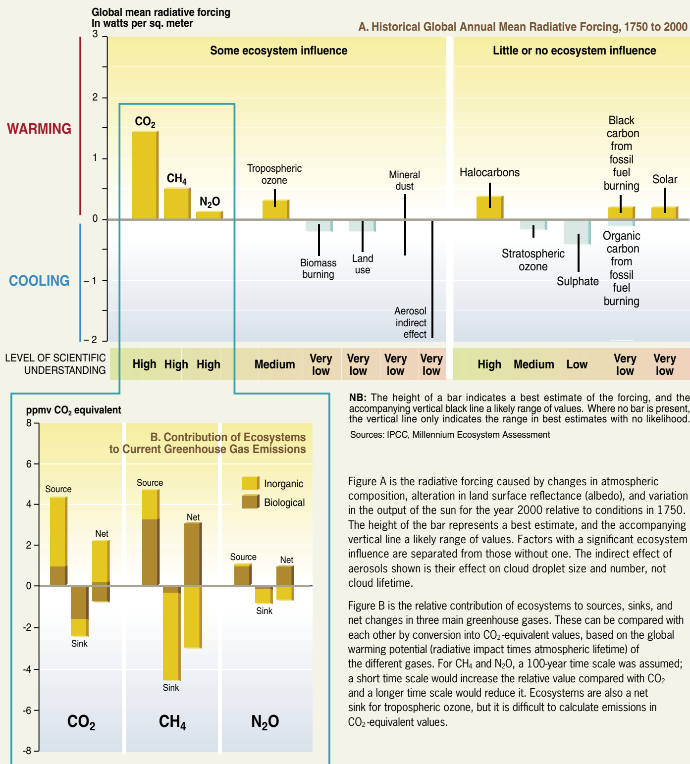
Appendix Figure A.6. CONTRIBUTION OF ECOSYSTEMS TO HISTORICAL RADIATIVE FORCING AND CURRENT GREENHOUSE GAS EMISSIONS (C13 Fig 13.3)
