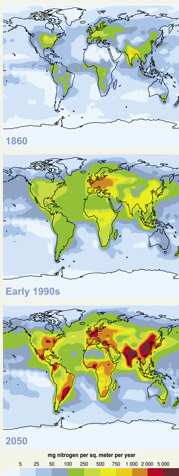
Figure 1.6. ESTIMATED TOTAL REACTIVE NITROGEN DEPOSITION FROM THE ATMOSPHERE (WET AND DRY) IN 1860, EARLY 1990S, AND PROJECTED FOR 2050 (milligrams of nitrogen per square meter per year) (R9 Fig 9.2)
